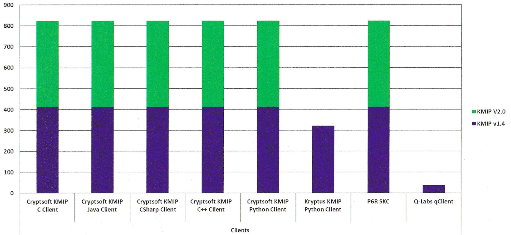
KMIP Client Test Results by KMIP Version - April 2018
